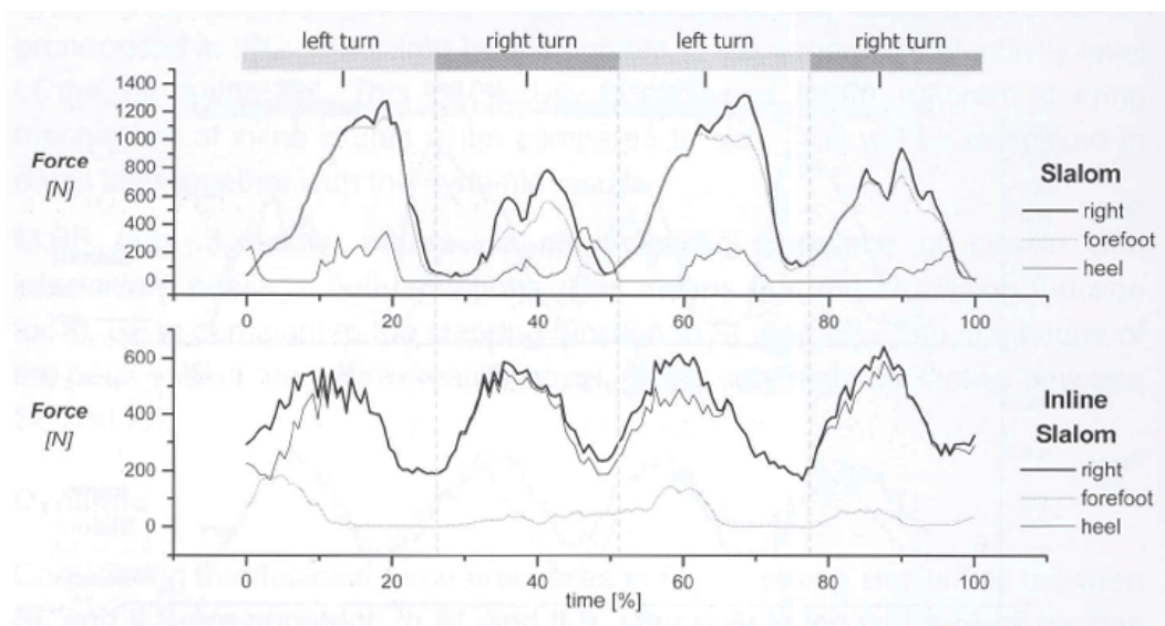
Figure 4 Dynamic characteristics - power distribution for front (forefoot) and back (heel) foot SL and ISL (short lines at the top of the diagram - the moment of passing the gate, dashed line - the ending of turn and passing to a new one) (Kroll et al., 2005)
