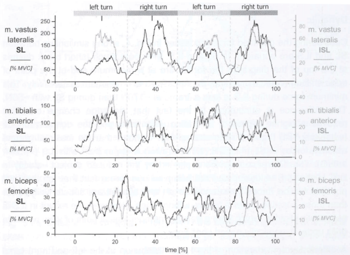
Figure 2 EMG activity of m.VL, TA, BF of the right leg in all three phases of the turn of the SL and ISL (short line at the top of the chart - the moment of crossing gates, dashed line - the ending of turn and passing to a new one) (Kroll et al., 2005)
